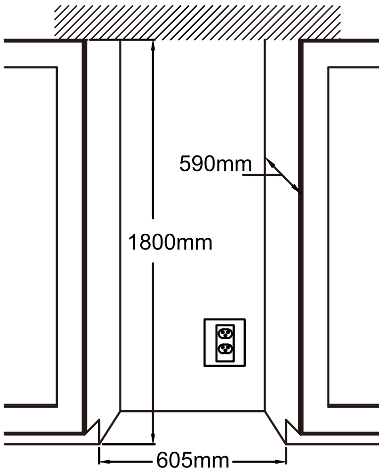
Cabinet Cut-Out
