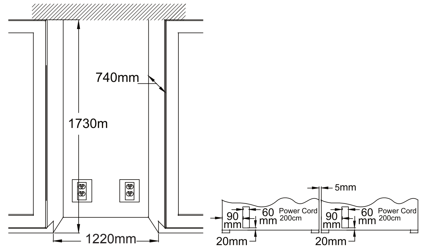
Cabinet Cut-Out
