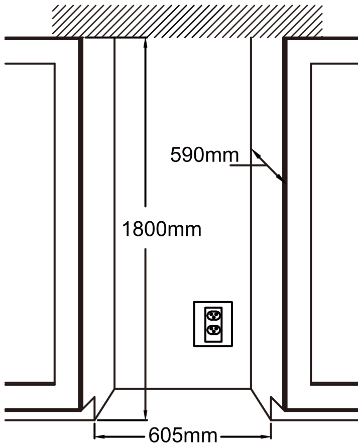
Cabinet Cut-Out
