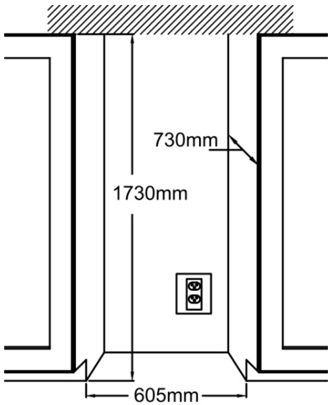
Cabinet Cut-Out
